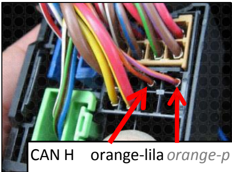
CAN-Abgriff am orig. Radio stecker Tap CAN on the orig. headunit connector
