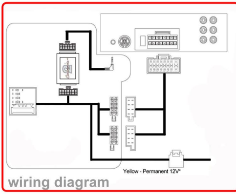
locate car wiring
